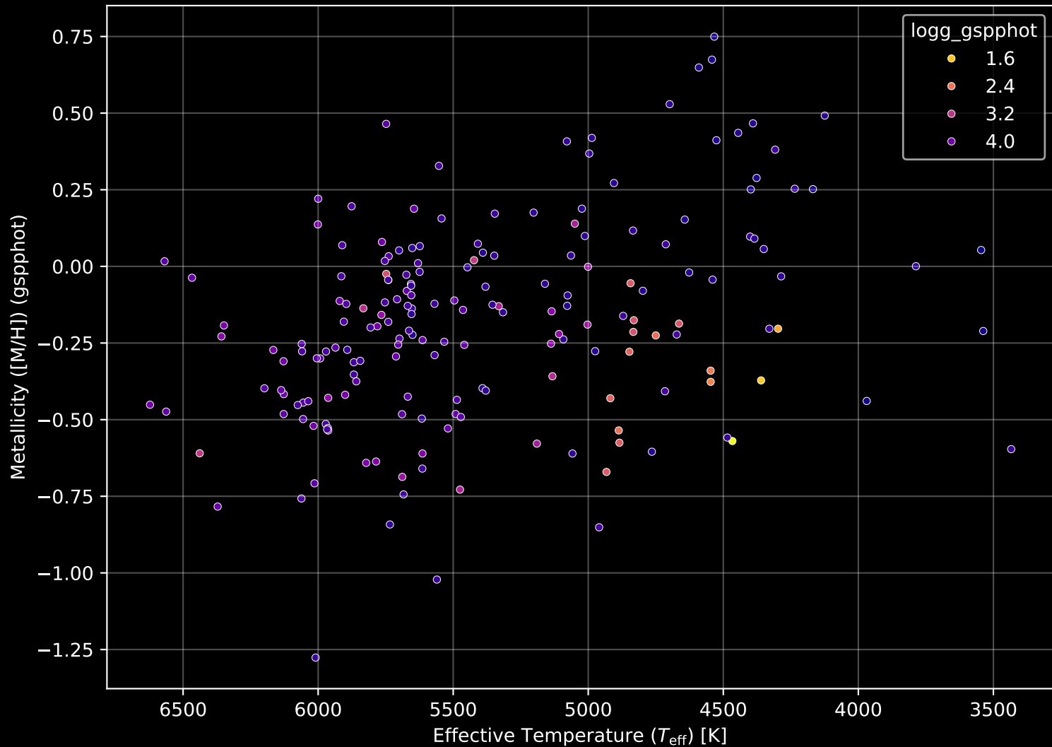
APOGEE DR17 Field: [124+67_MGA] Stellar Population Parameters (n= 189)
