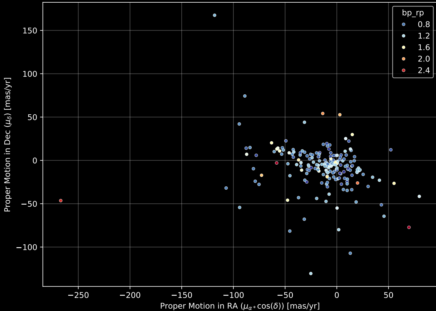
APOGEE DR17 Field: [124+67_MGA] Proper Motion Diagram (n= 189)
