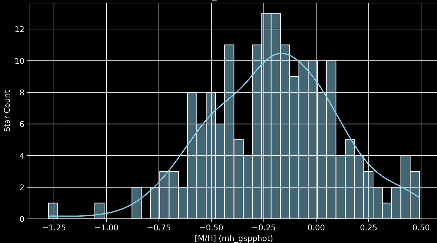
APOGEE DR17 Field: [124+67_MGA [M/H] (mh_gspphot) (n= 185)
